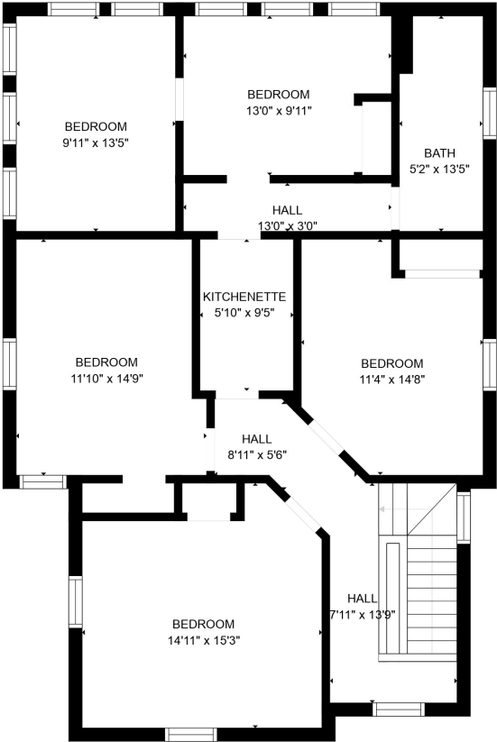
FLOOR 3
