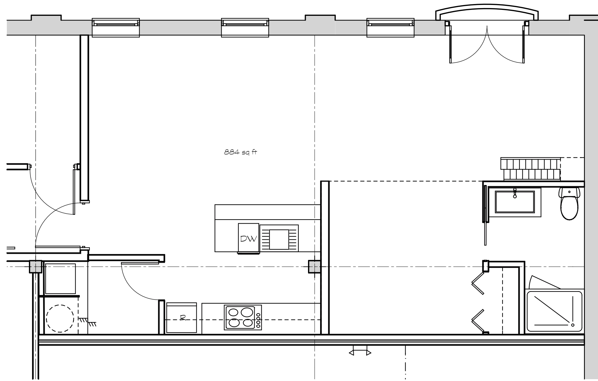
1 1ST FLR APARTMENT SCALE: 1/4" = 1'-0"
