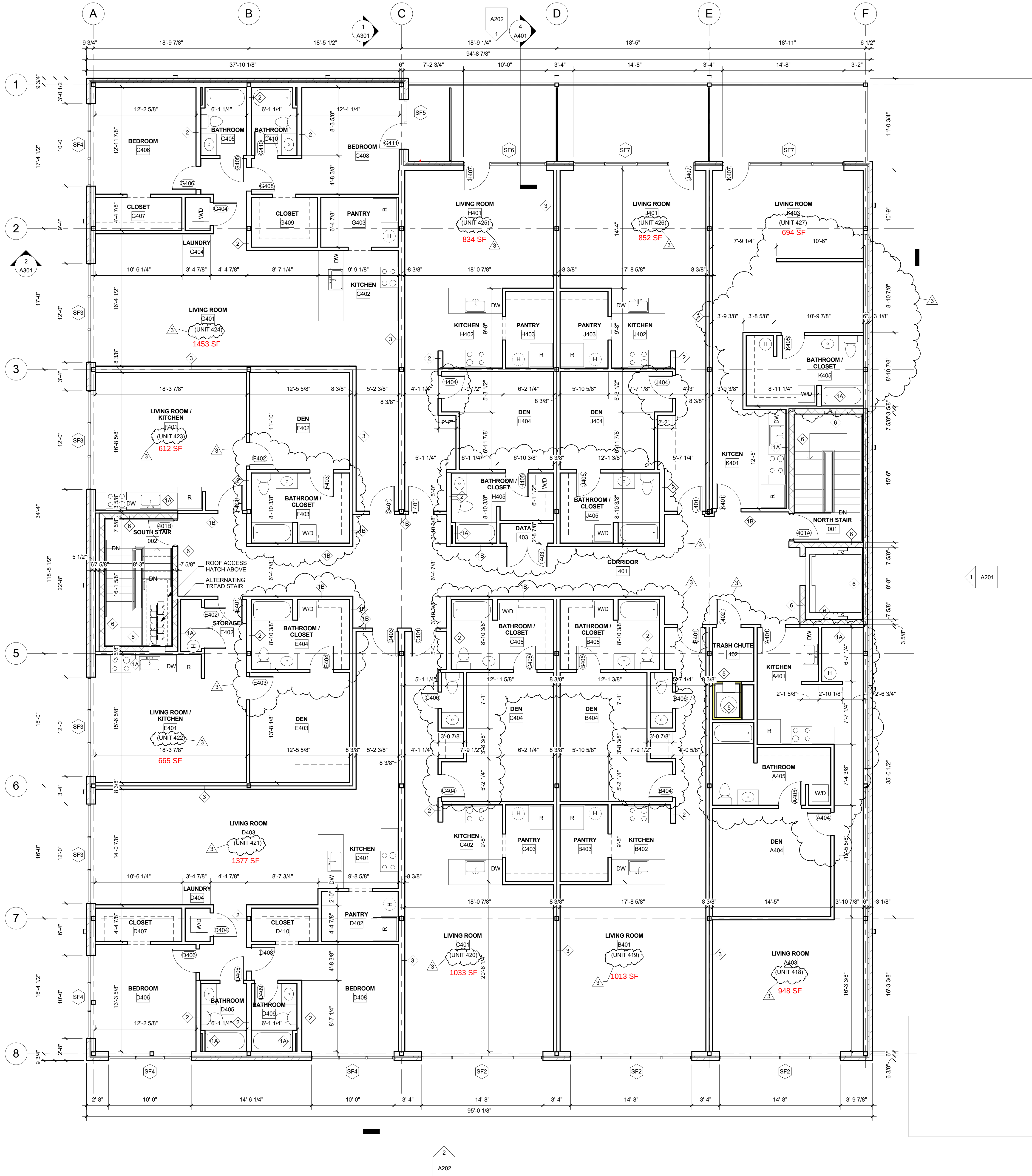
1 LEVEL 4 FLOOR PLAN 3/16" = 1'-0"
